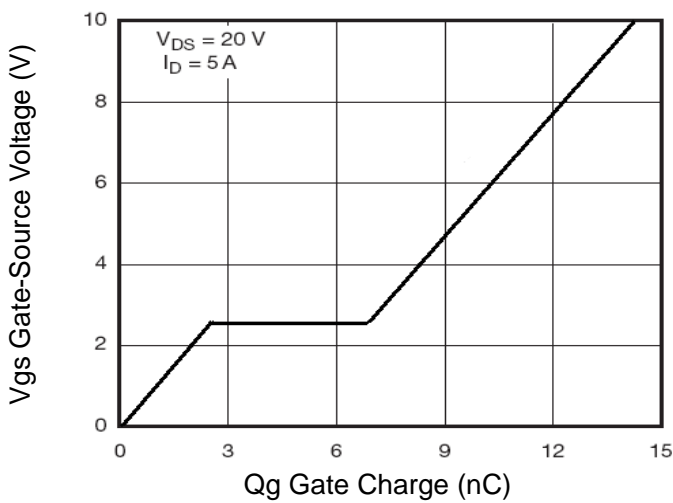
Figure 11 Gate Charge
