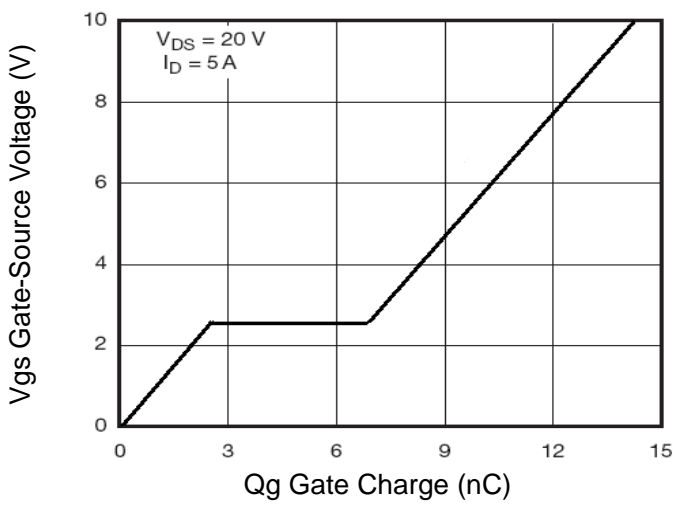
Figure 11 Gate Charge
