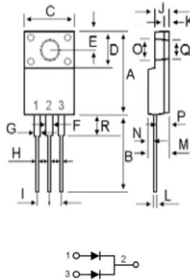
TO-220F PACKAGE
